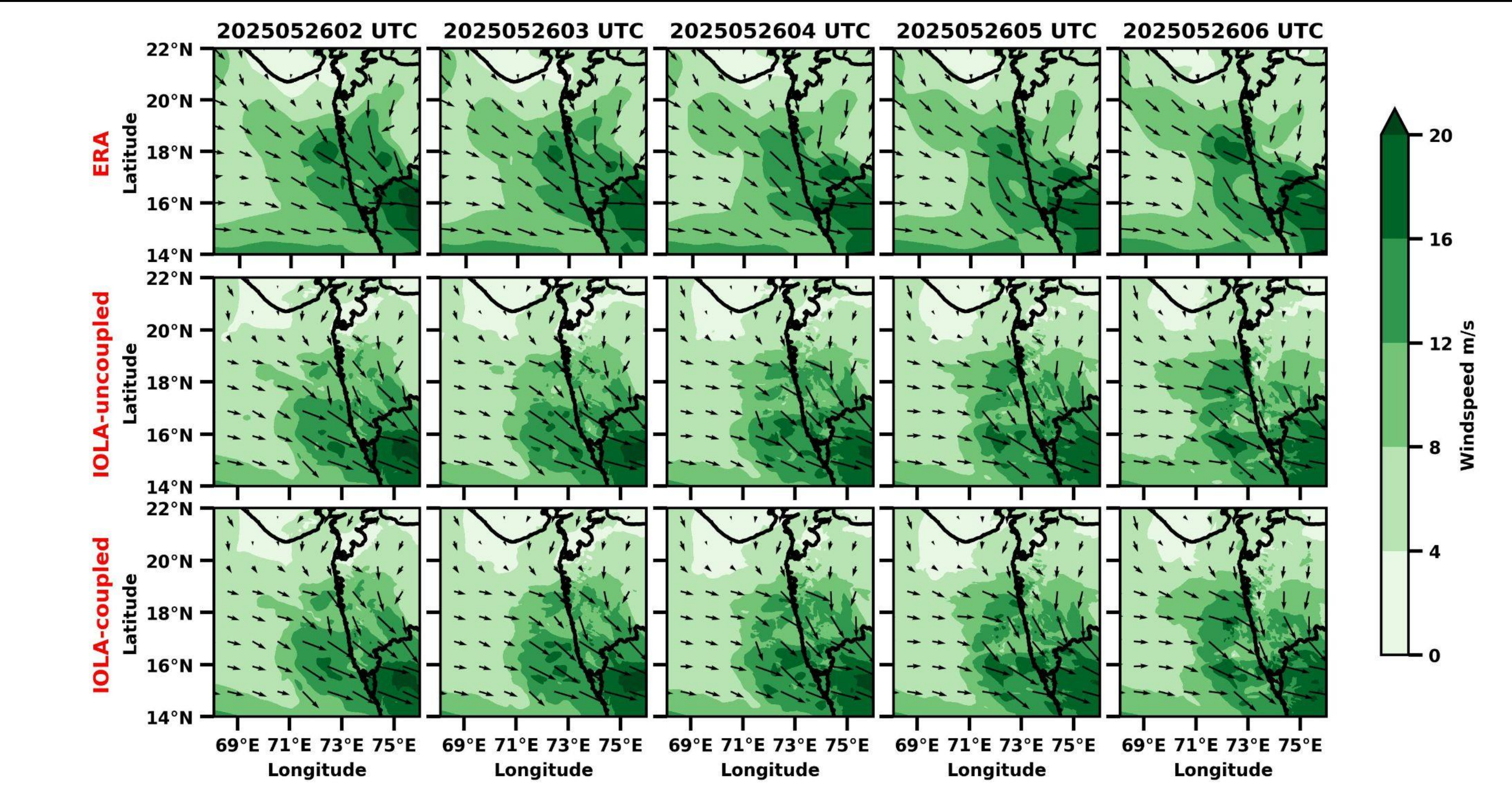
Fig 6. ERA re-analysis and IOLA simulated 850 hPa winds during time period ( \pm 2 hrs) of cloudburst events in both cases. Green Shade represents wind speed and arrow represents wind direction.
