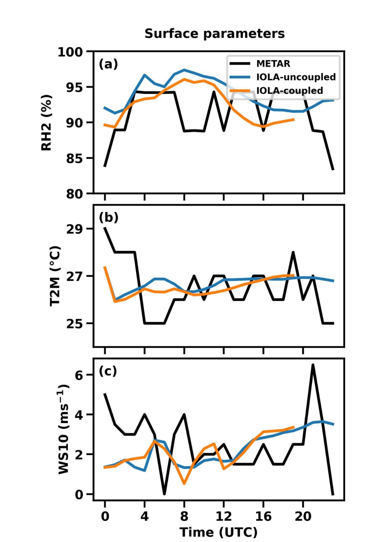
Fig 5. Intercomparison of IOLA uncoupled and coupled model simulated surface parameters; (a) 2m Relative humidity (RH2, %), (b) 2m Temperature (T2M, °C), (c) 10m Wind Speed (WS10; ms-1) for the Mumbai case of 2025 May 26.
