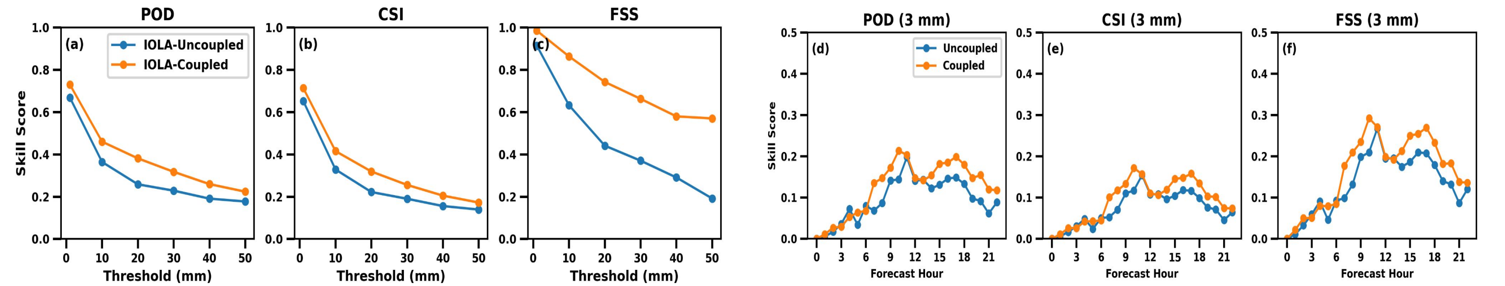
Fig 3. Mean skill scores (a) Probability of Detection (POD), (b) Critical Success Index (CSI), and (c) Fraction Skill Score (FSS) from IOLA-uncoupled and IOLA-coupled simulations compared against GPM. Similar to (a), (b), (c), but for a 3 mm threshold at different forecast hours.
