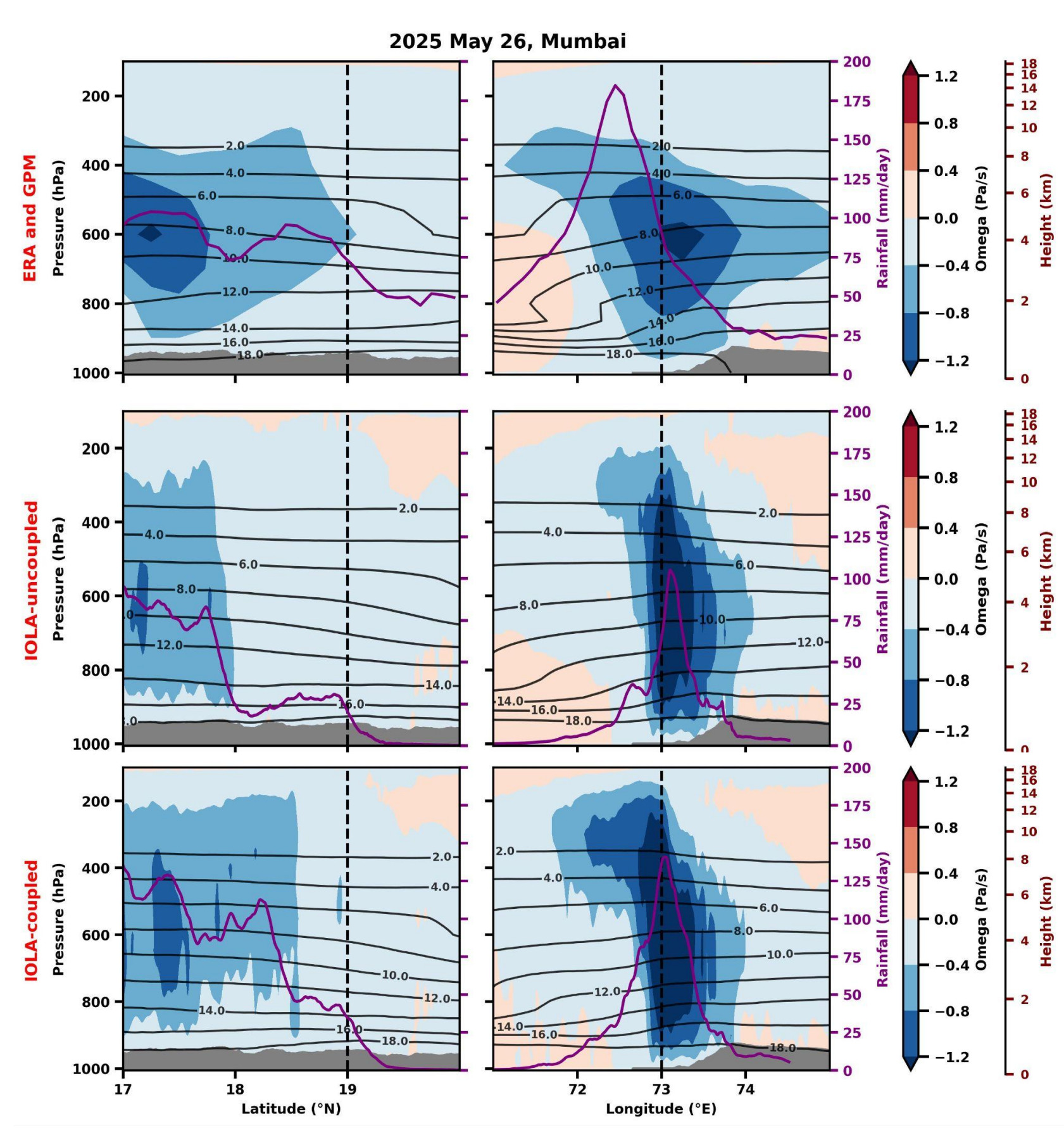
Fig 4. Pressure-latitude plot of Specific Humidity (contour; g/kg) and omega (shaded; Pa/s) averaged over longitude. The rainfall (mm/day) is averaged and presented along the latitude in the (purple) line plot, and values are presented in the Secondary Y-axis. The black dashed line represents the latitude of Mumbai. The right-hand side figure is a similar Pressure-longitude plot, but for Specific Humidity (contour; g/kg) and omega (shaded; Pa/s) are averaged over latitudes, while the dashed line represents the longitude of Mumbai. The plot is shown from ERA-reanalysis-GPM (1st row), IOLA uncoupled model simulated (2nd row) and 3rd IOLA coupled model simulated.
